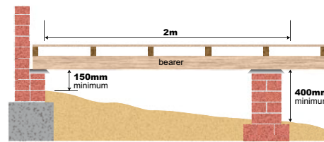
BCA Minimum underfloor clearance requirements
